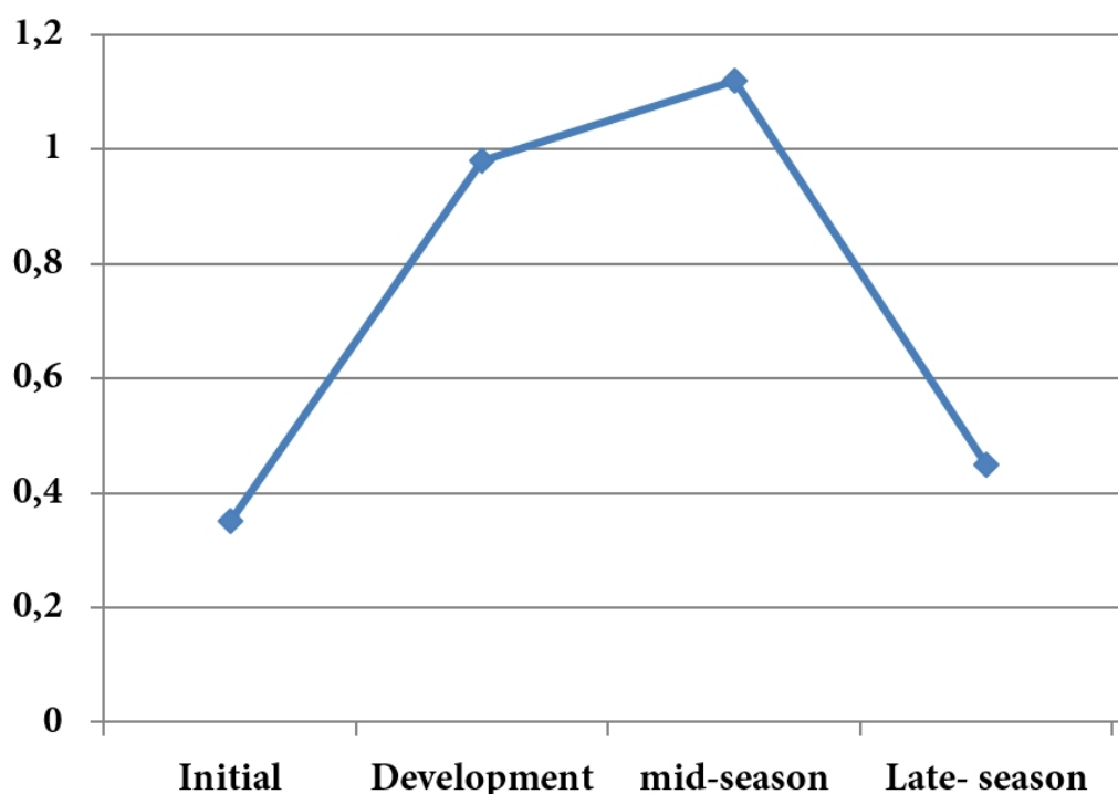
Figure 2: The 2-year average crop coefficient (Kc) values of maize (cultivar T.W.C. 321) during different growth stage
